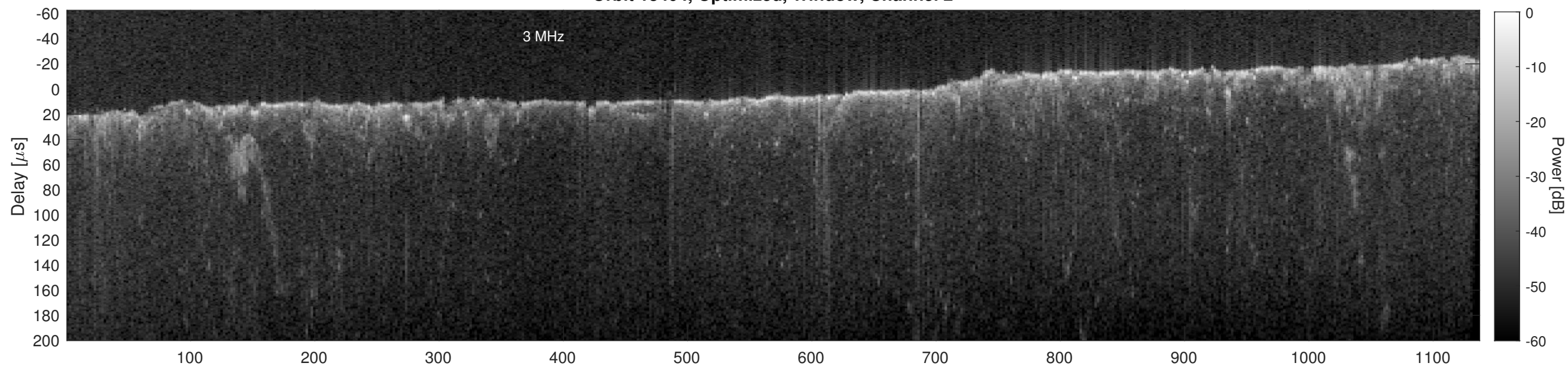
Orbit 13404, Cluttergram
