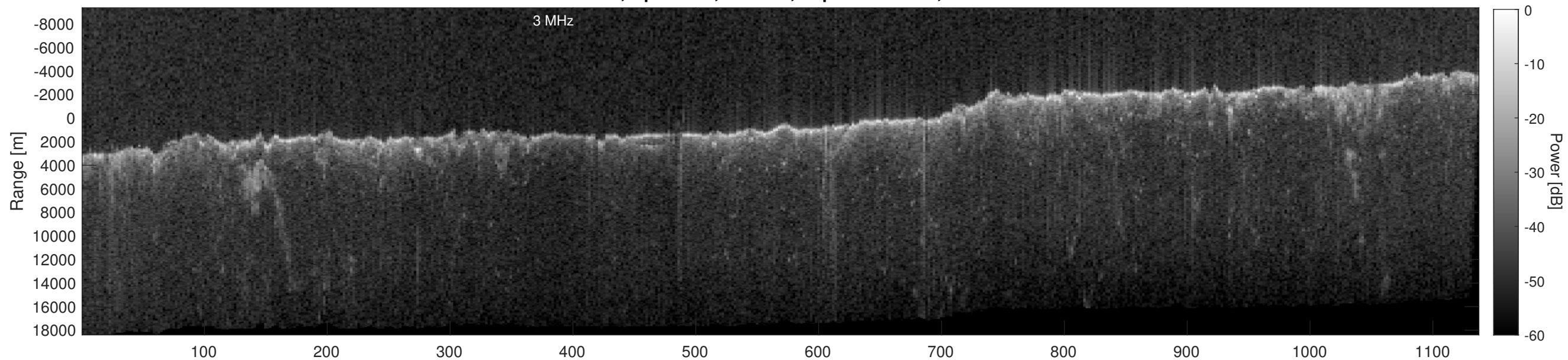
Orbit 13404, Depth-Corrected Cluttergram
