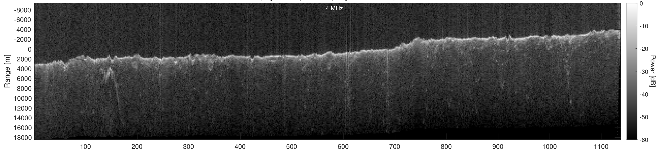
Orbit 13404, Optimized, Window, Depth-Corrected, Channel 2
