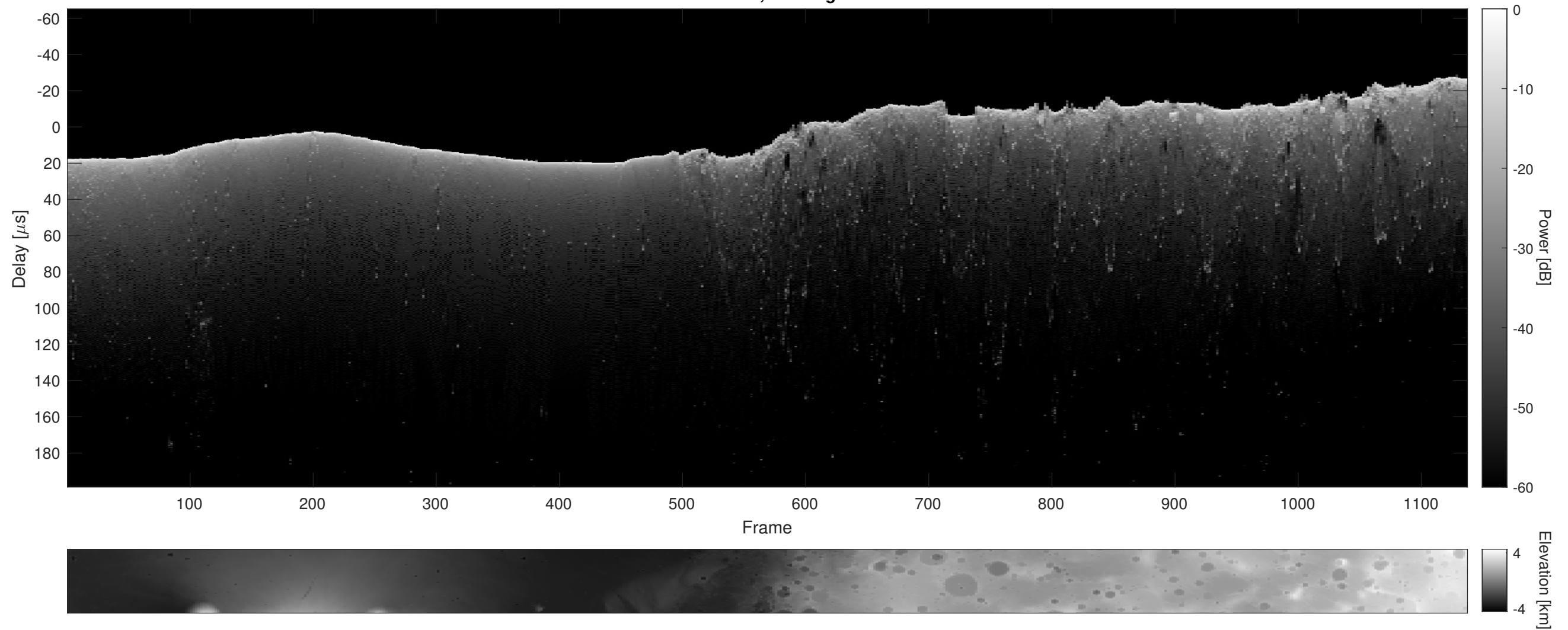
Orbit 13406, Cluttergram
