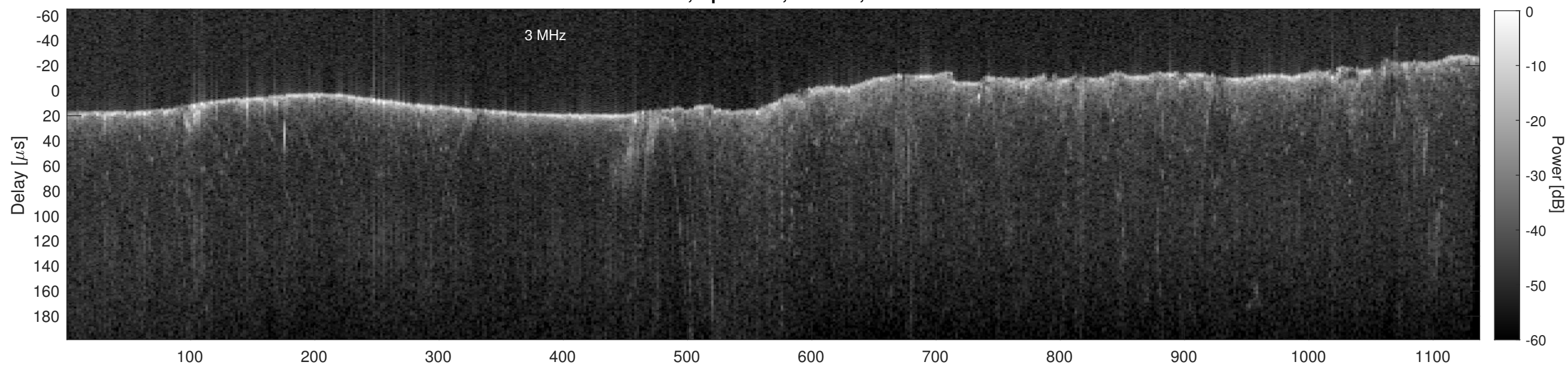
Orbit 13406, Cluttergram
