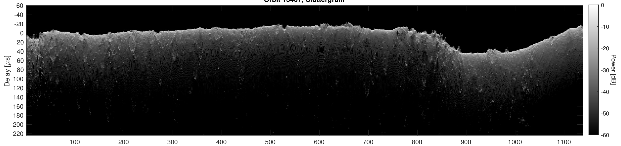
Orbit 13407, Cluttergram
