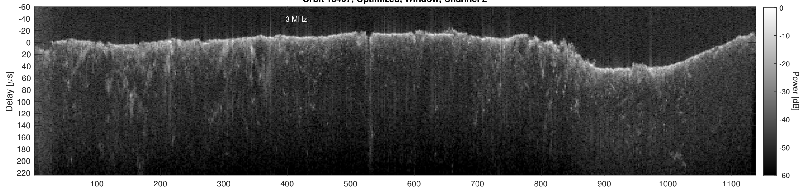
Orbit 13407, Cluttergram
