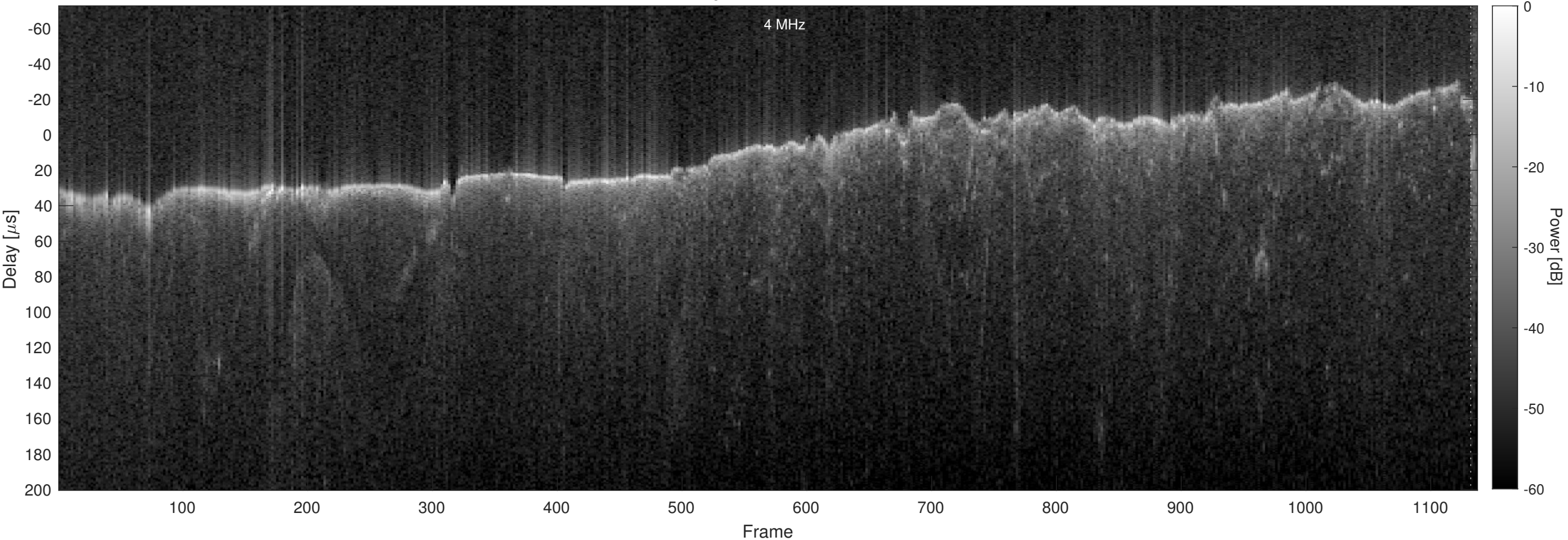
Orbit 13409, Chapman, No Window, Channel 2
