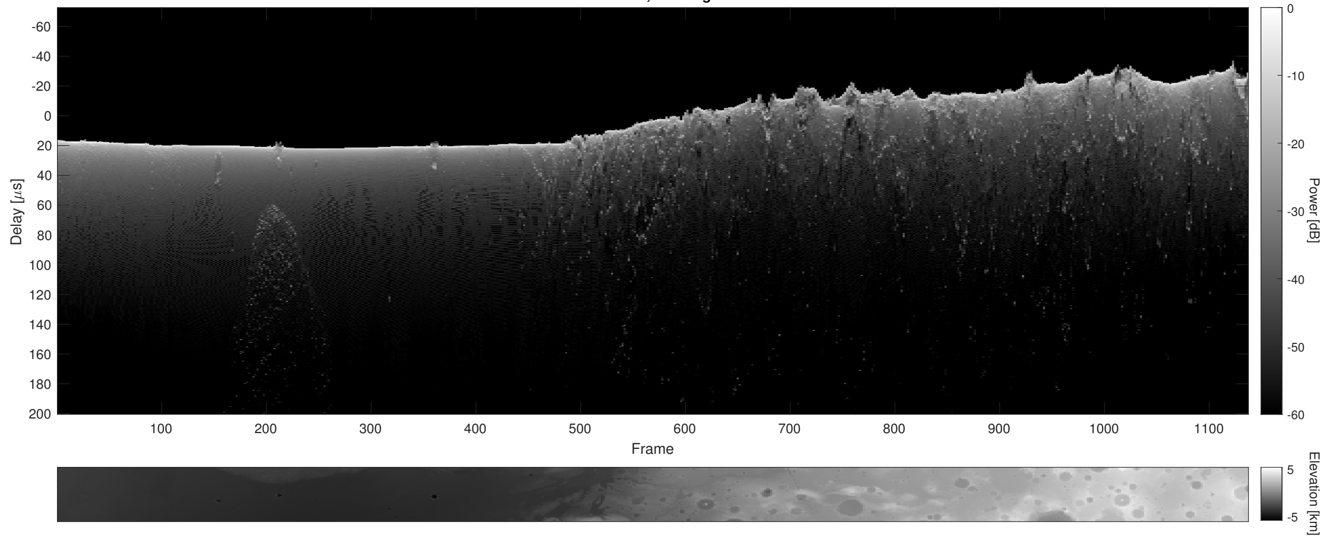
Orbit 13409, Cluttergram
