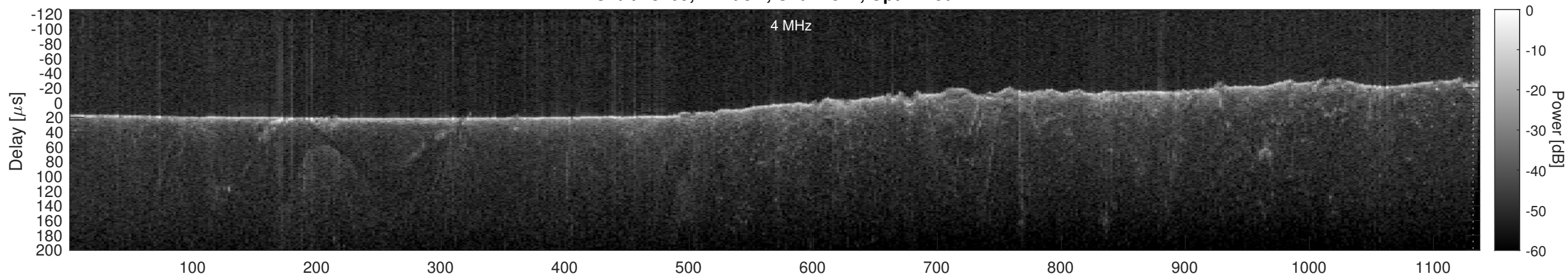
Orbit 13409, Cluttergram
