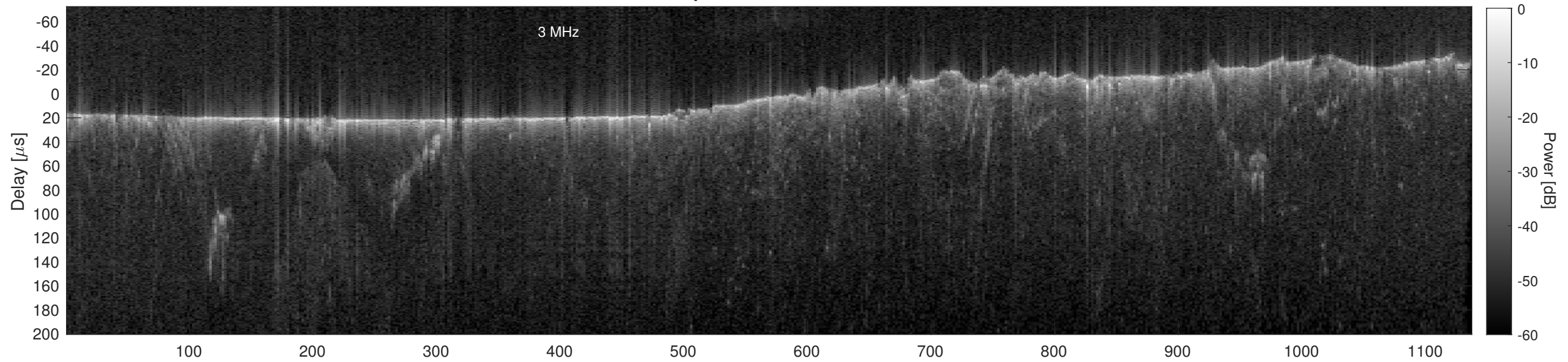
Orbit 13409, Cluttergram
