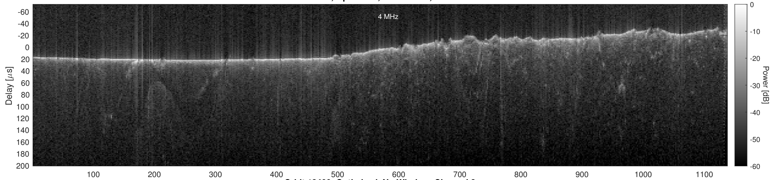
Orbit 13409, Optimized, No Window, Channel 2
