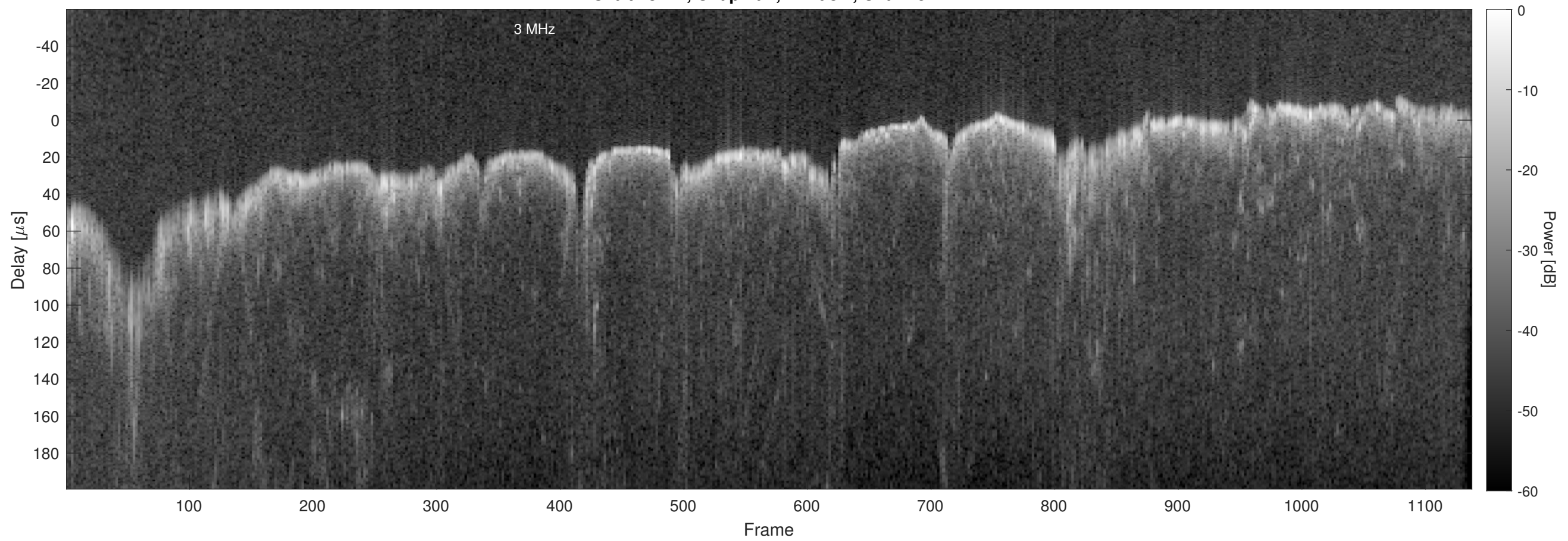
Orbit 13411, Chapman, Window, Channel 2
