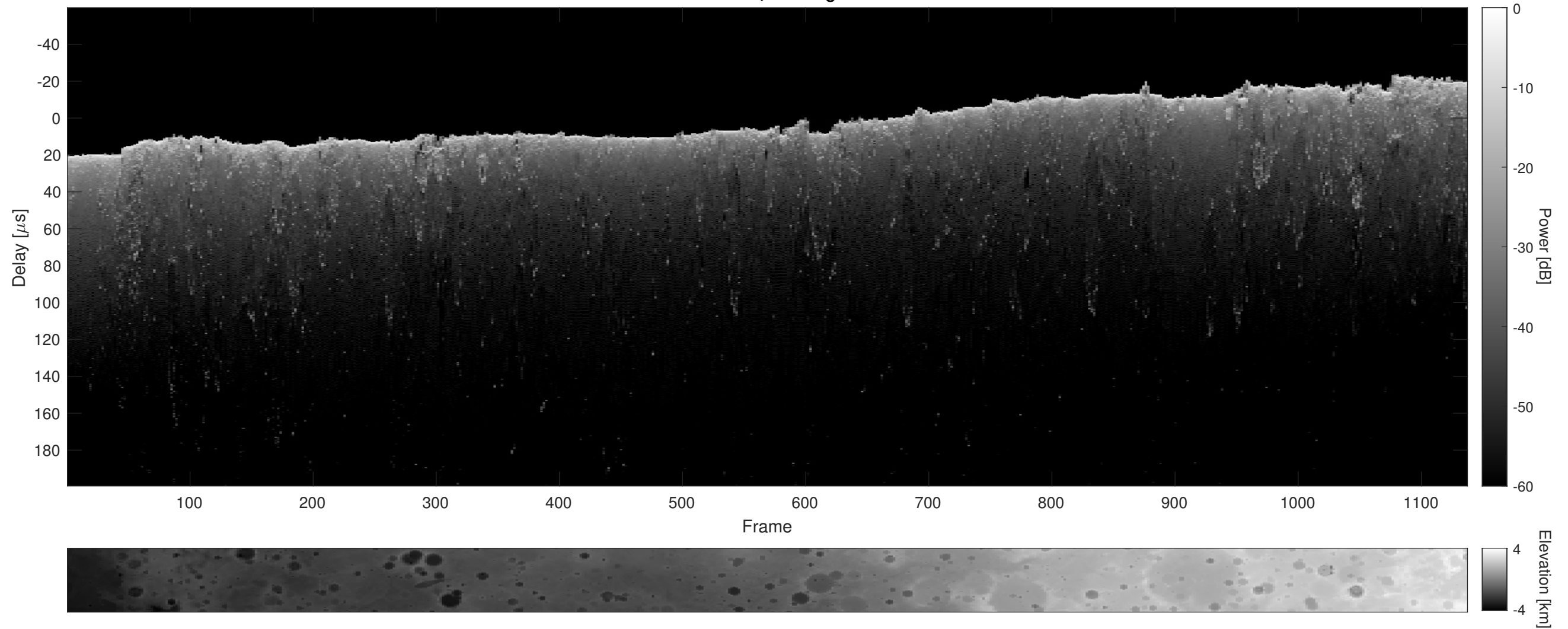
Orbit 13411, Cluttergram
