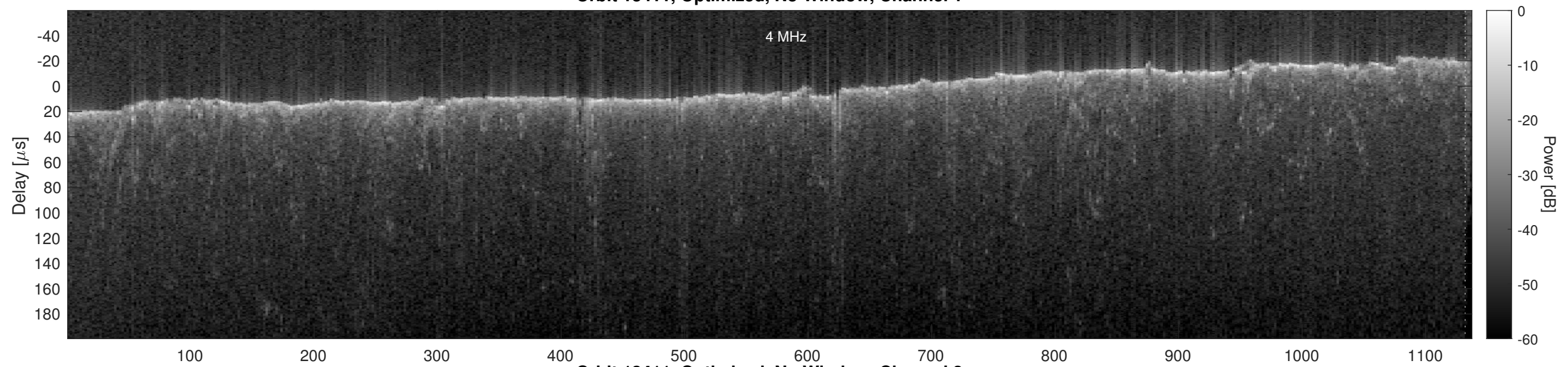
Orbit 13411, Optimized, No Window, Channel 2
