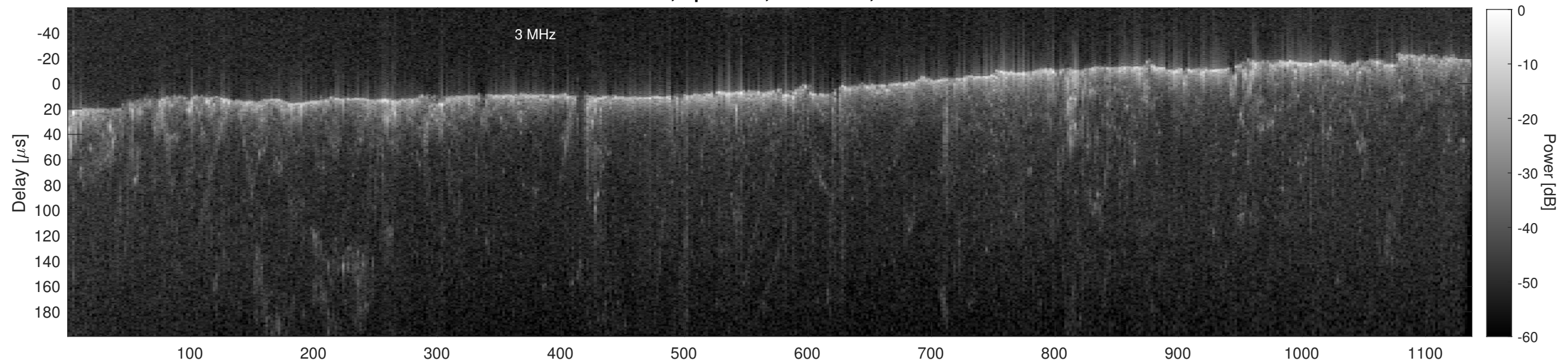
Orbit 13411, Cluttergram
