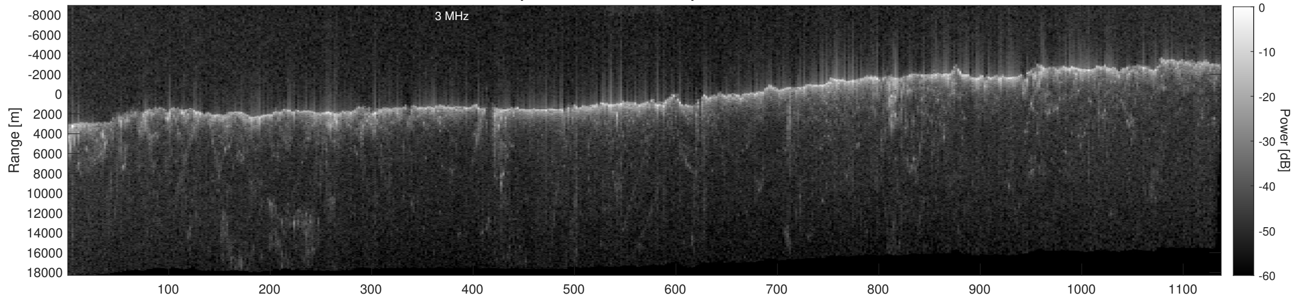
Orbit 13411, Depth-Corrected Cluttergram
