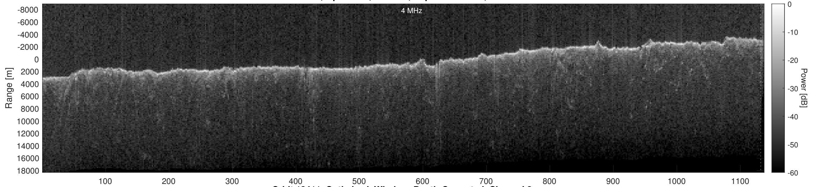
Orbit 13411, Optimized, Window, Depth-Corrected, Channel 2
