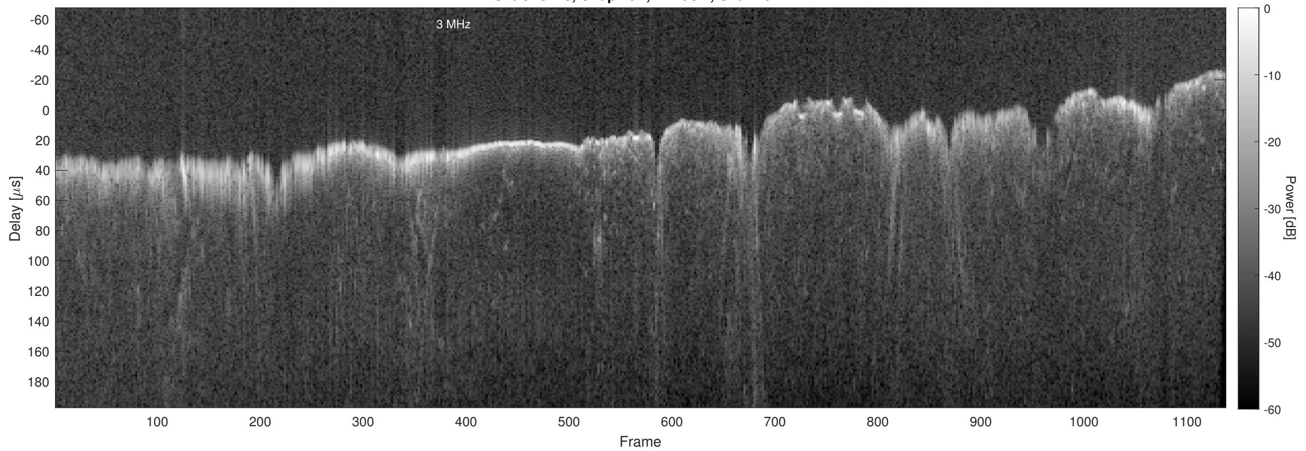
Orbit 13413, Chapman, Window, Channel 2
