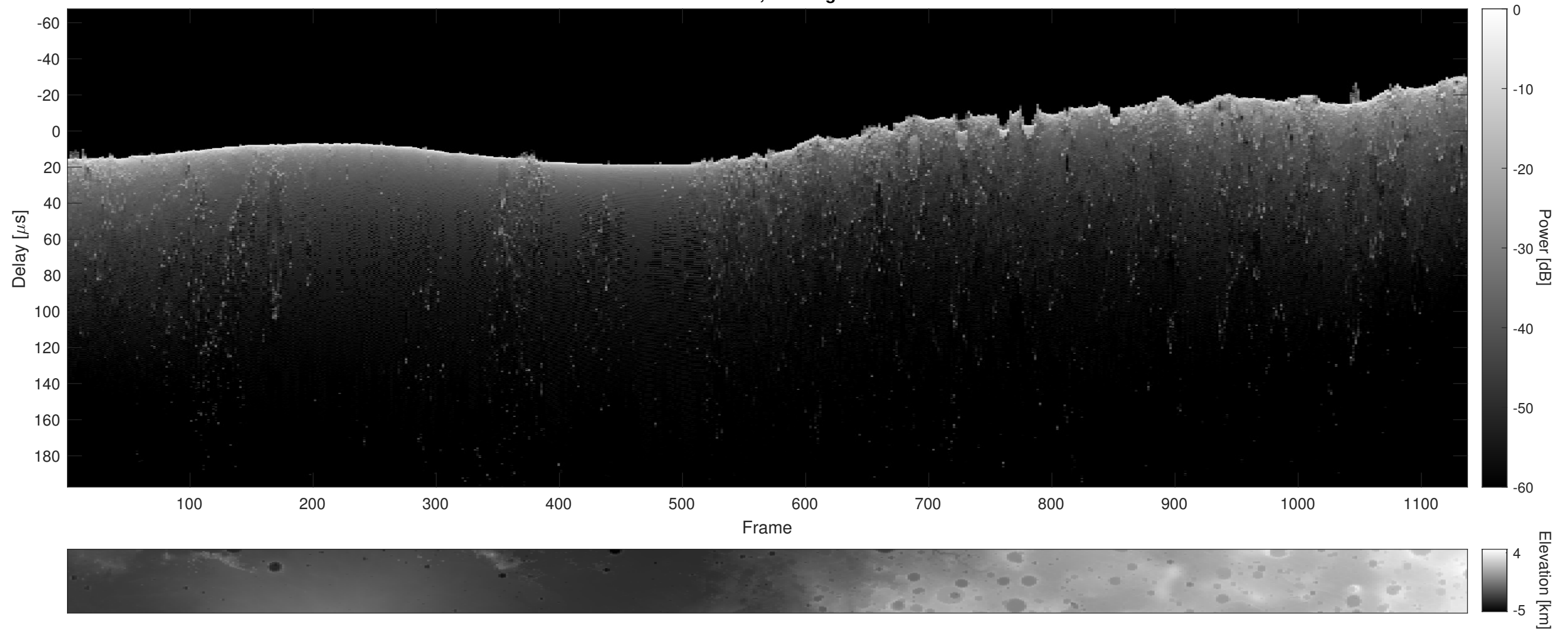
Orbit 13413, Cluttergram
