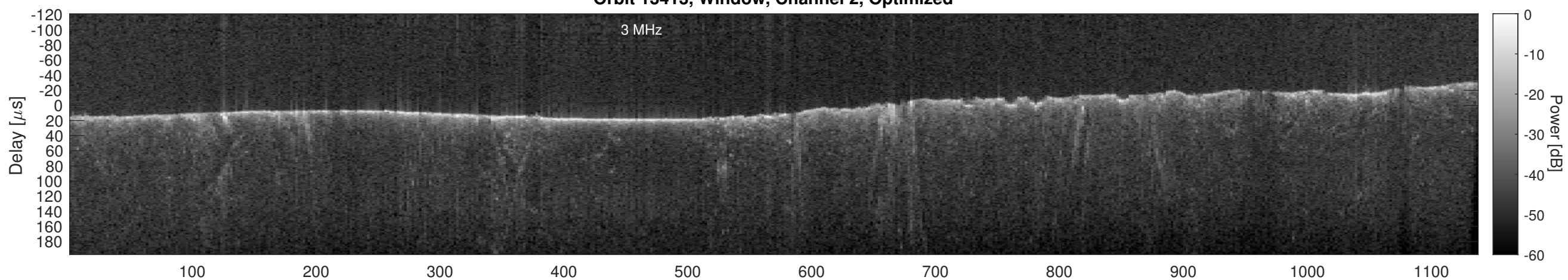
Orbit 13413, Cluttergram
