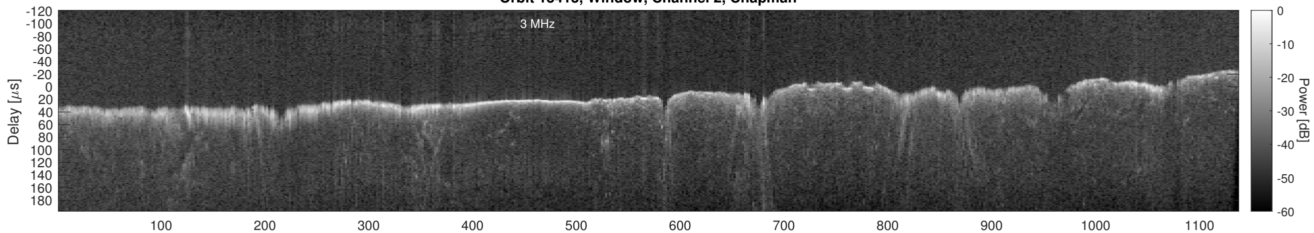
Orbit 13413, Window, Channel 2, Optimized
