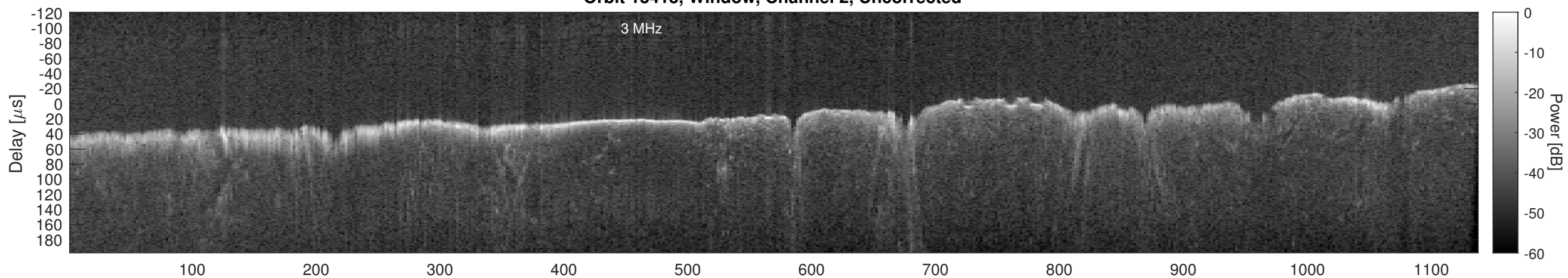
Orbit 13413, Window, Channel 2, Chapman
