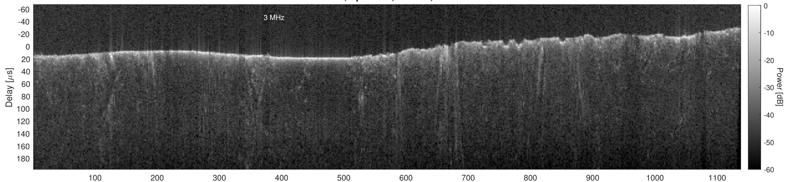
Orbit 13413, Cluttergram
