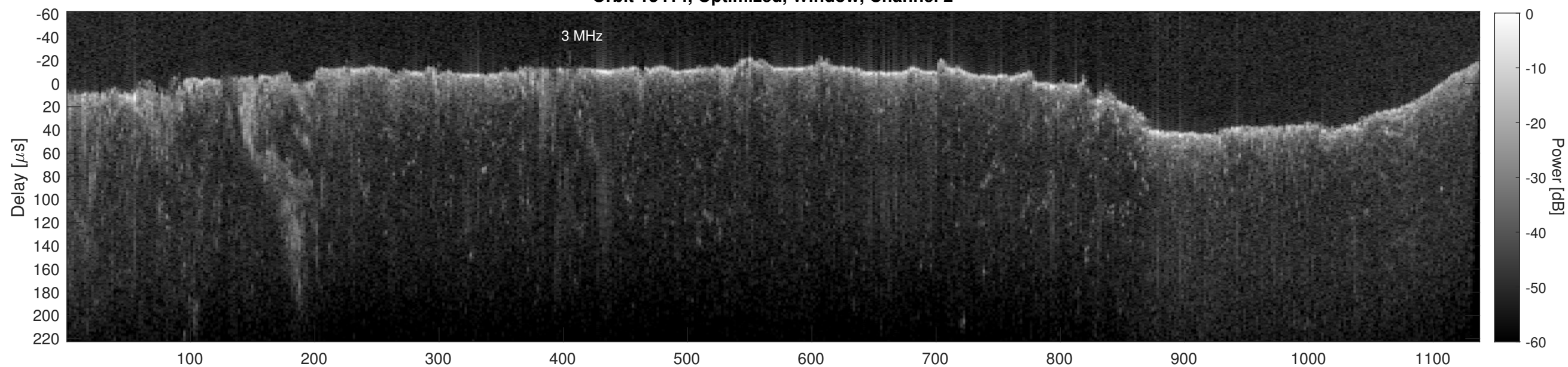
Orbit 13414, Cluttergram
