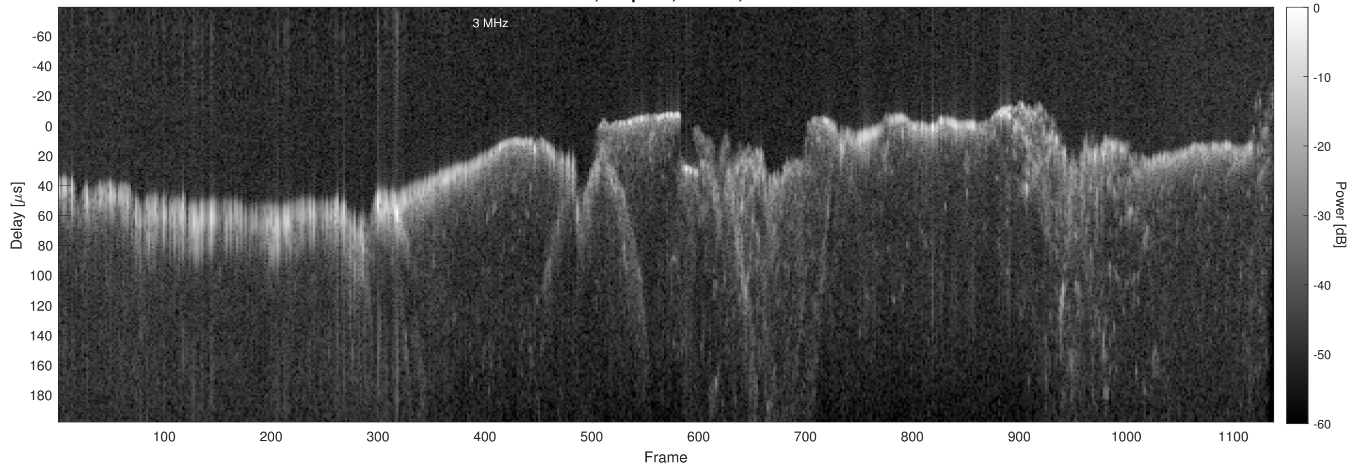
Orbit 13415, Chapman, Window, Channel 2
