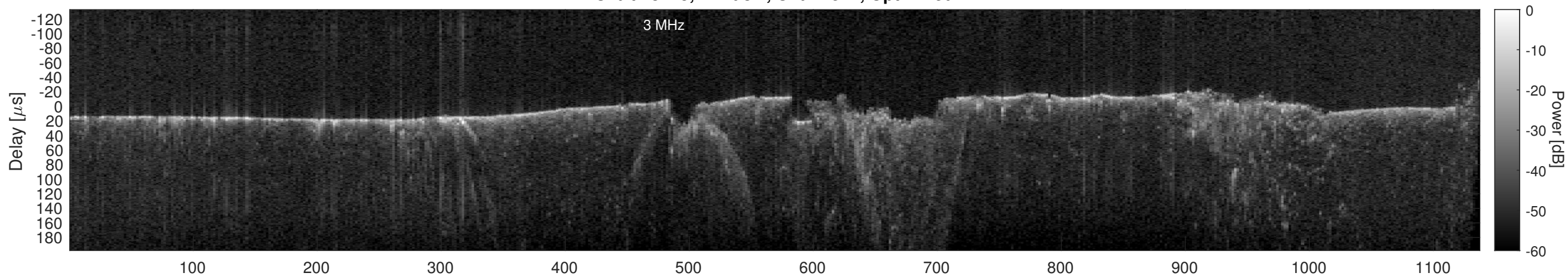
Orbit 13415, Cluttergram
