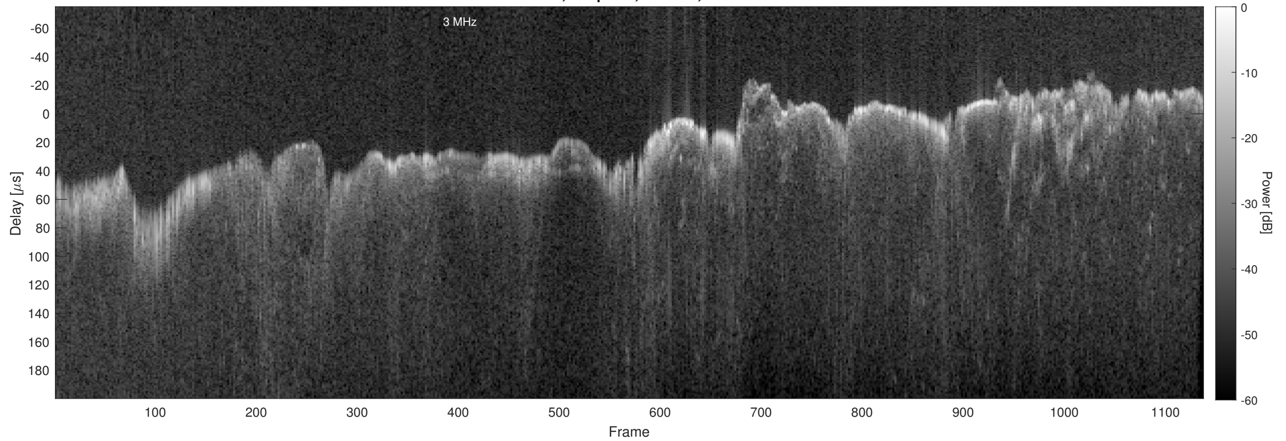
Orbit 13416, Chapman, Window, Channel 2
