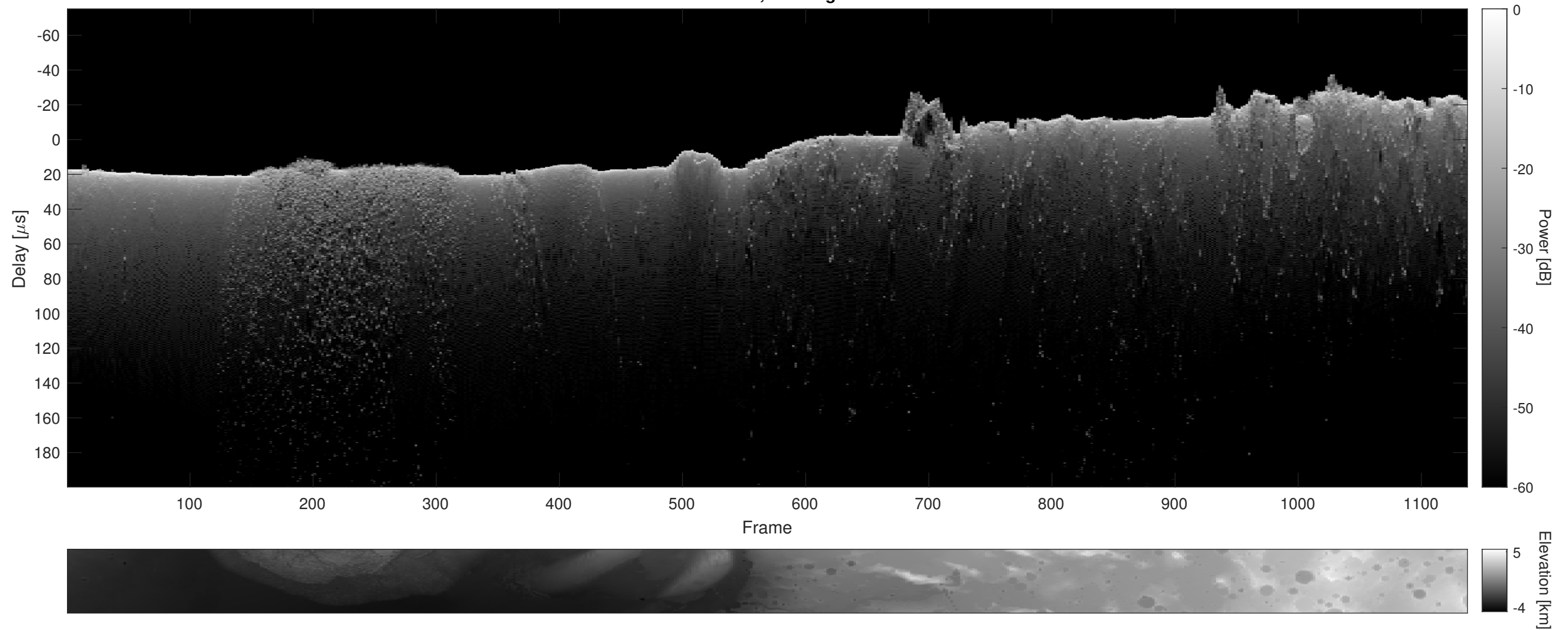
Orbit 13416, Cluttergram
