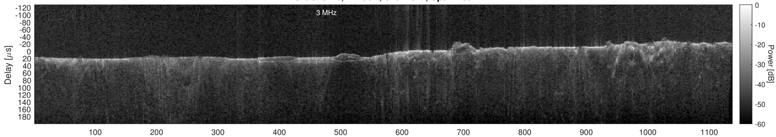
Orbit 13416, Cluttergram
