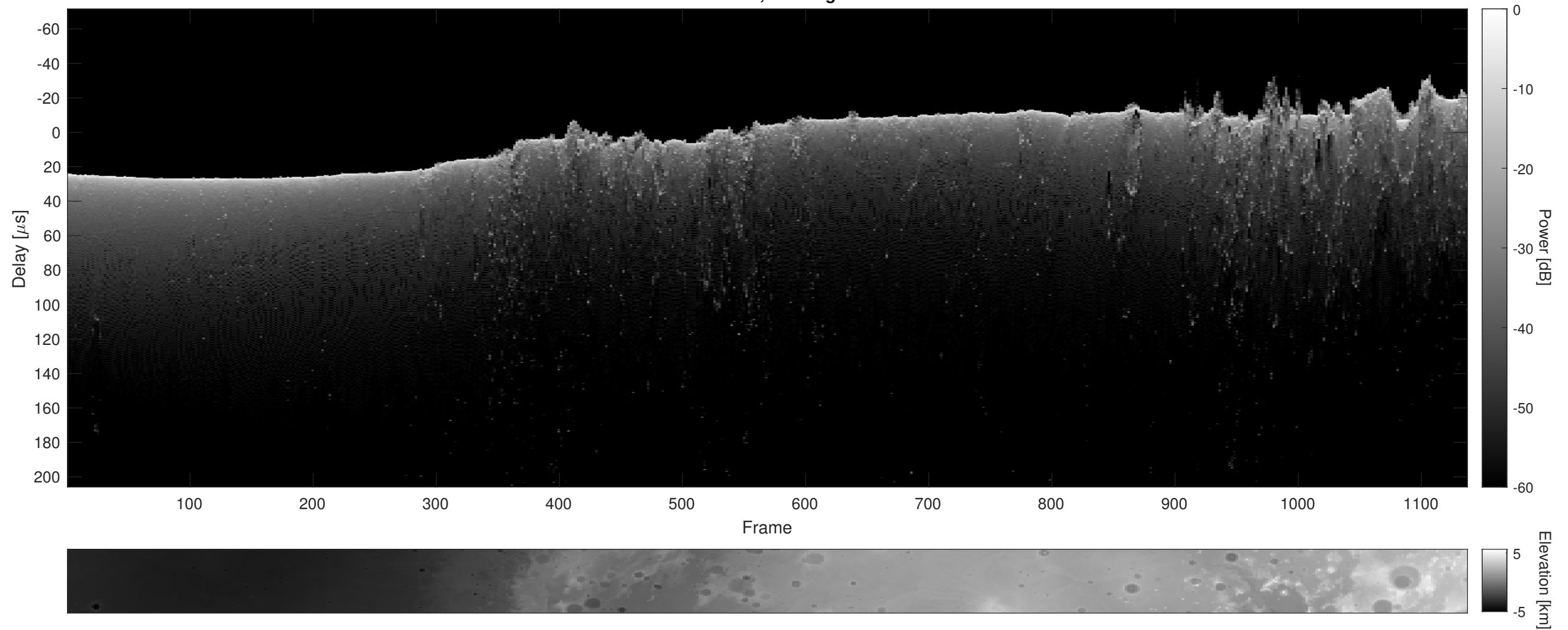
Orbit 13417, Cluttergram
