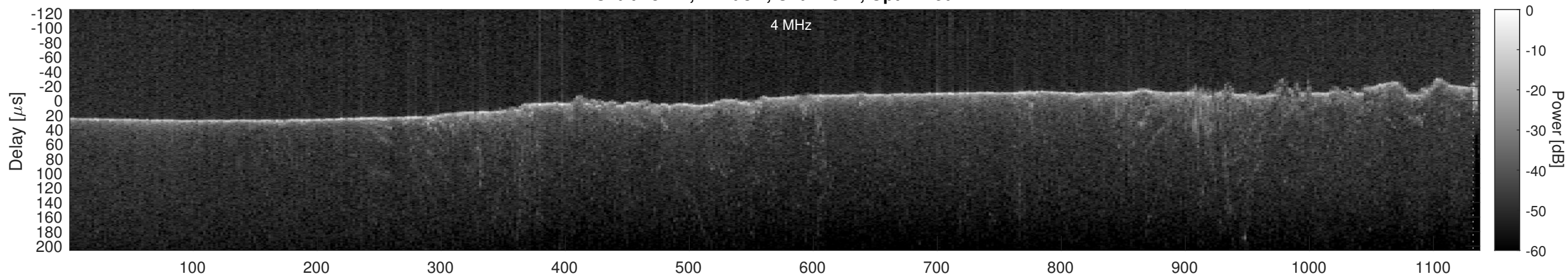
Orbit 13417, Cluttergram
