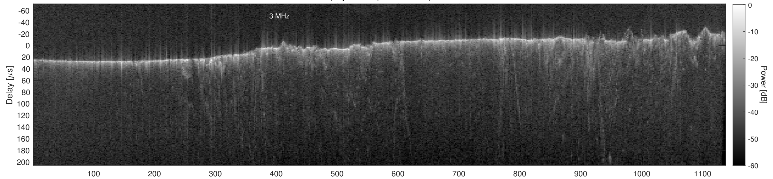
Orbit 13417, Cluttergram
