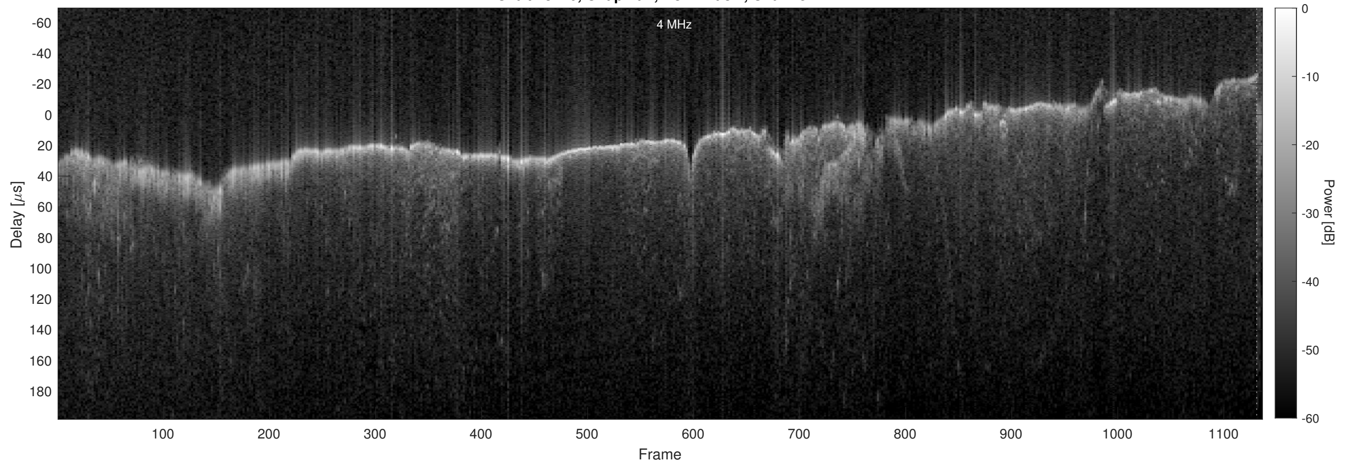
Orbit 13420, Chapman, No Window, Channel 2
