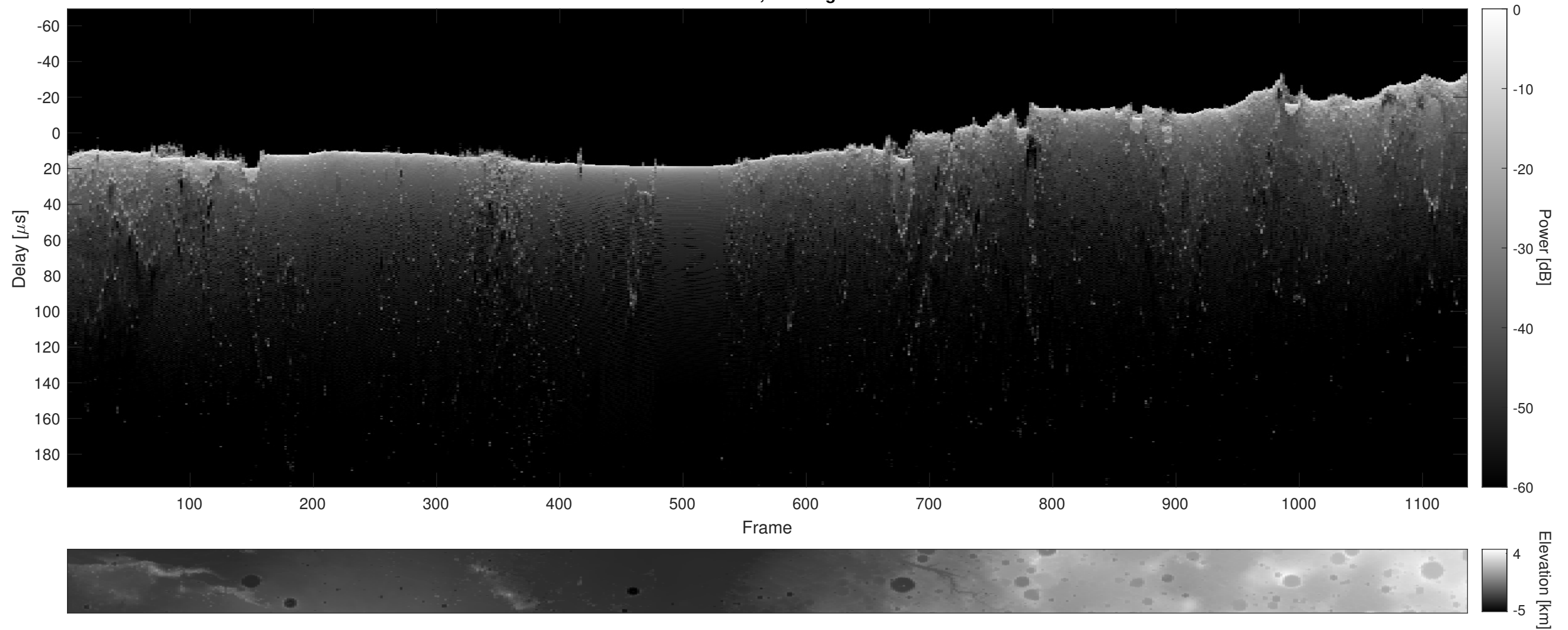
Orbit 13420, Cluttergram
