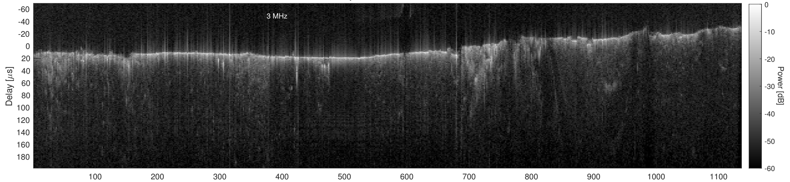
Orbit 13420, Cluttergram
