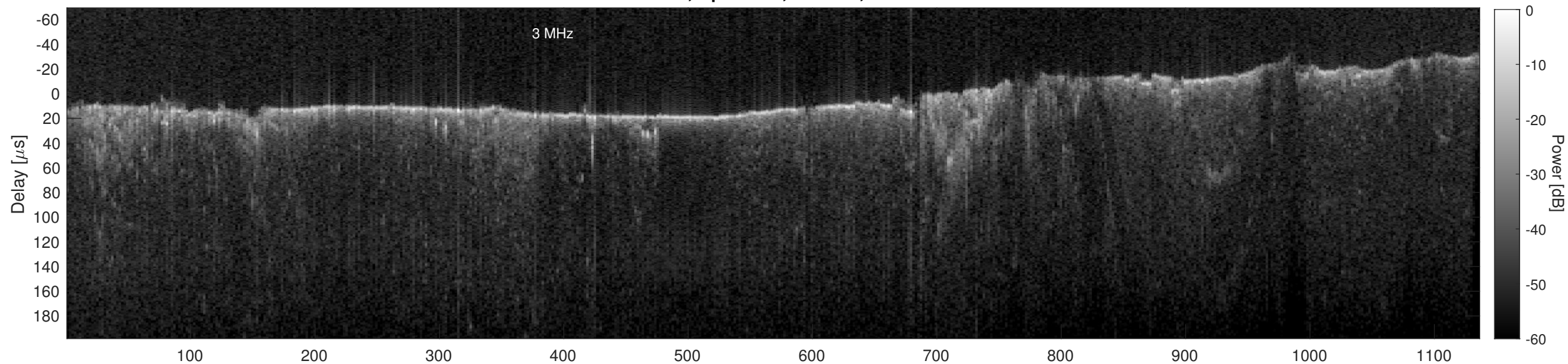
Orbit 13420, Cluttergram
