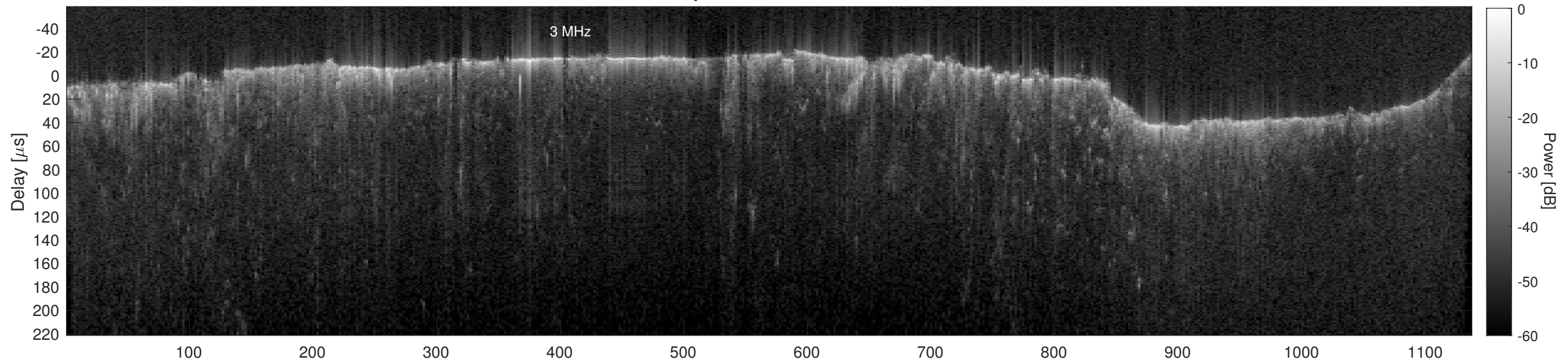
Orbit 13421, Cluttergram
