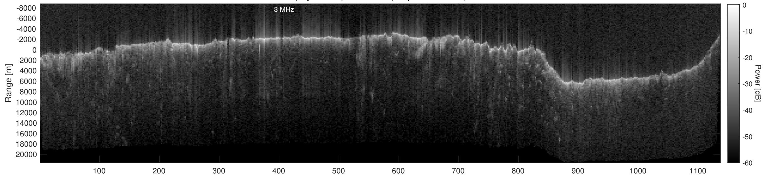
Orbit 13421, Depth-Corrected Cluttergram
