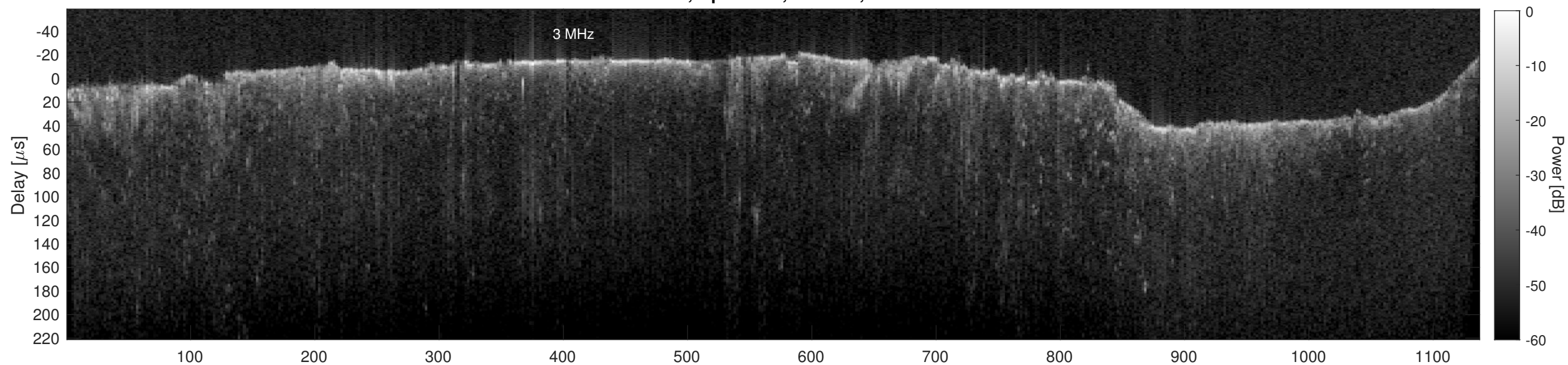
Orbit 13421, Cluttergram
