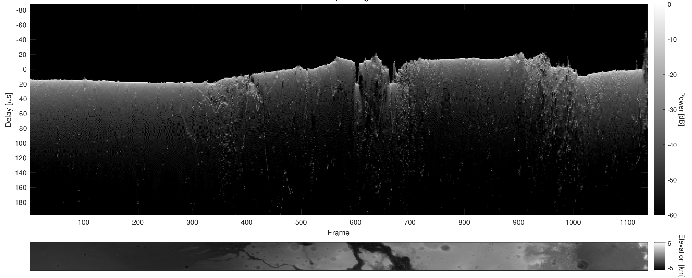
Orbit 13422, Cluttergram
