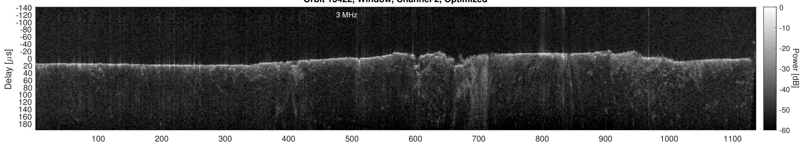
Orbit 13422, Cluttergram
