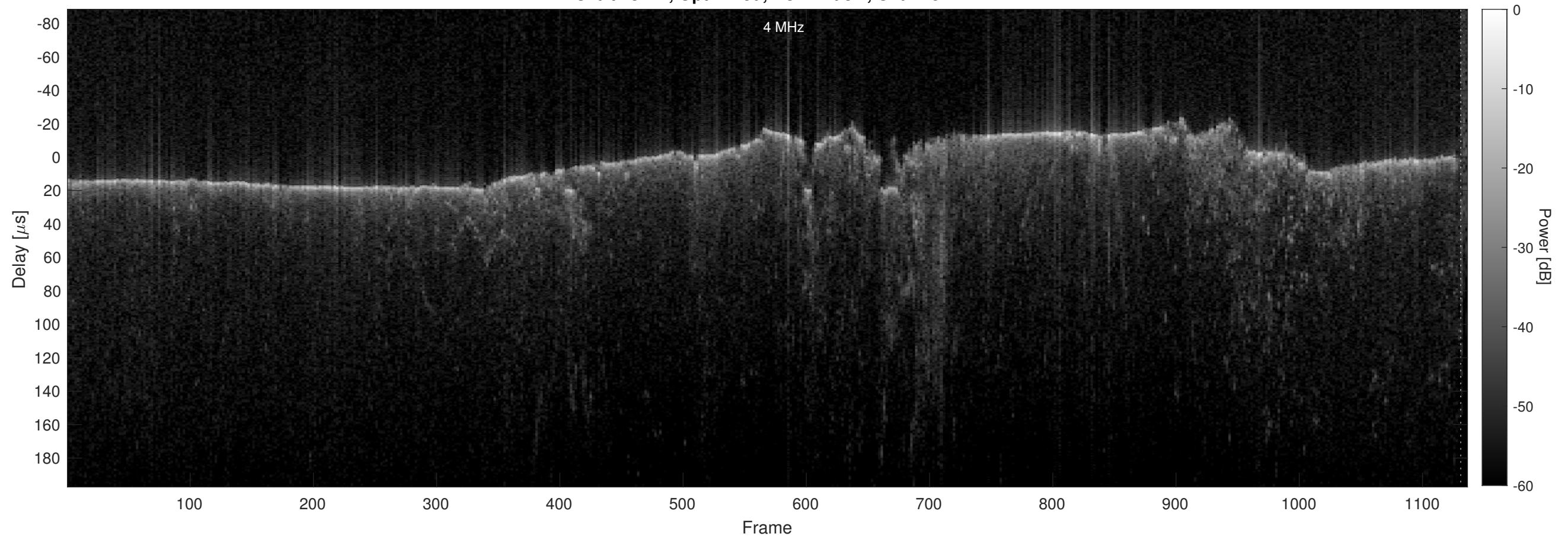
Orbit 13422, Optimized, No Window, Channel 2
