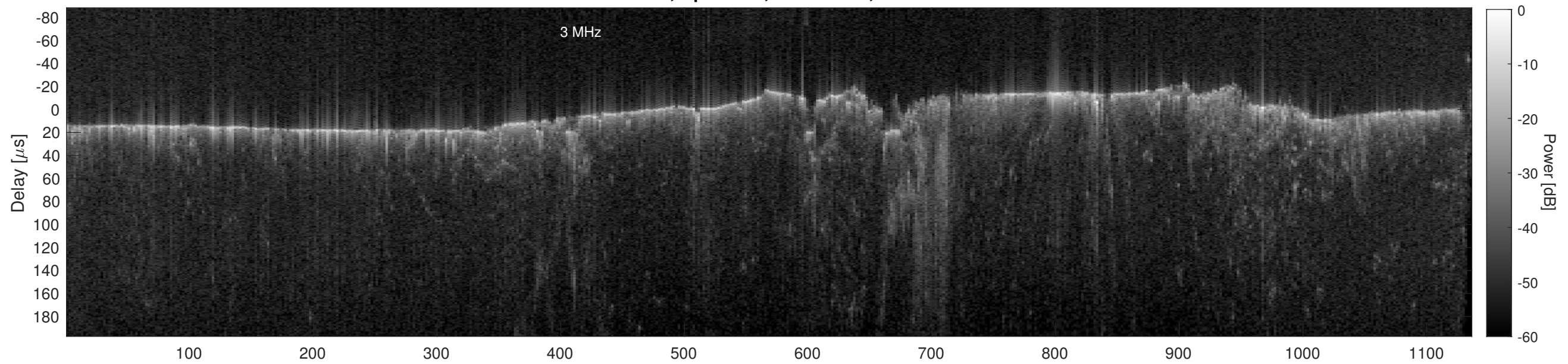
Orbit 13422, Cluttergram
