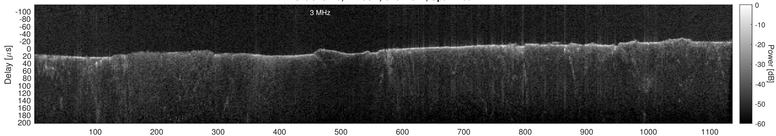
Orbit 13423, Cluttergram
