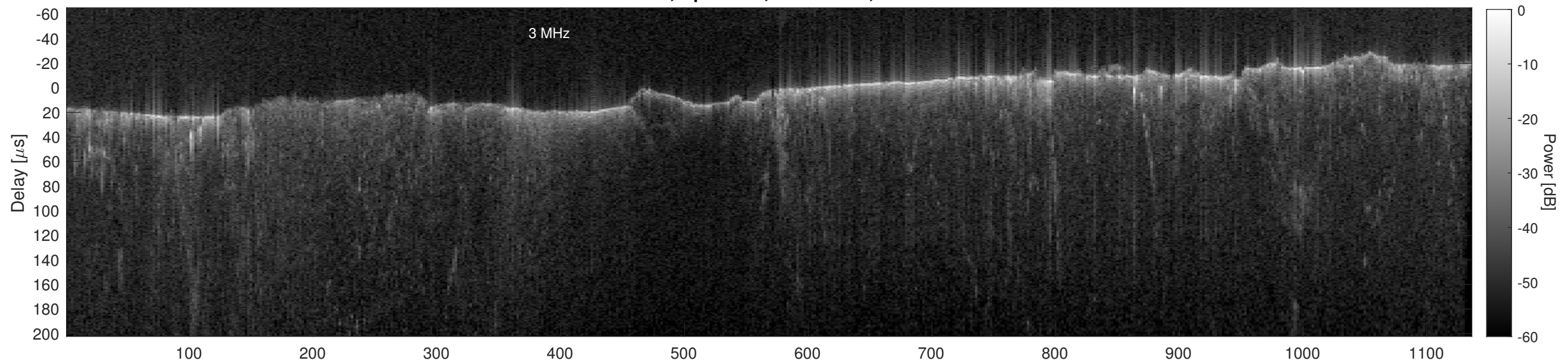
Orbit 13423, Cluttergram
