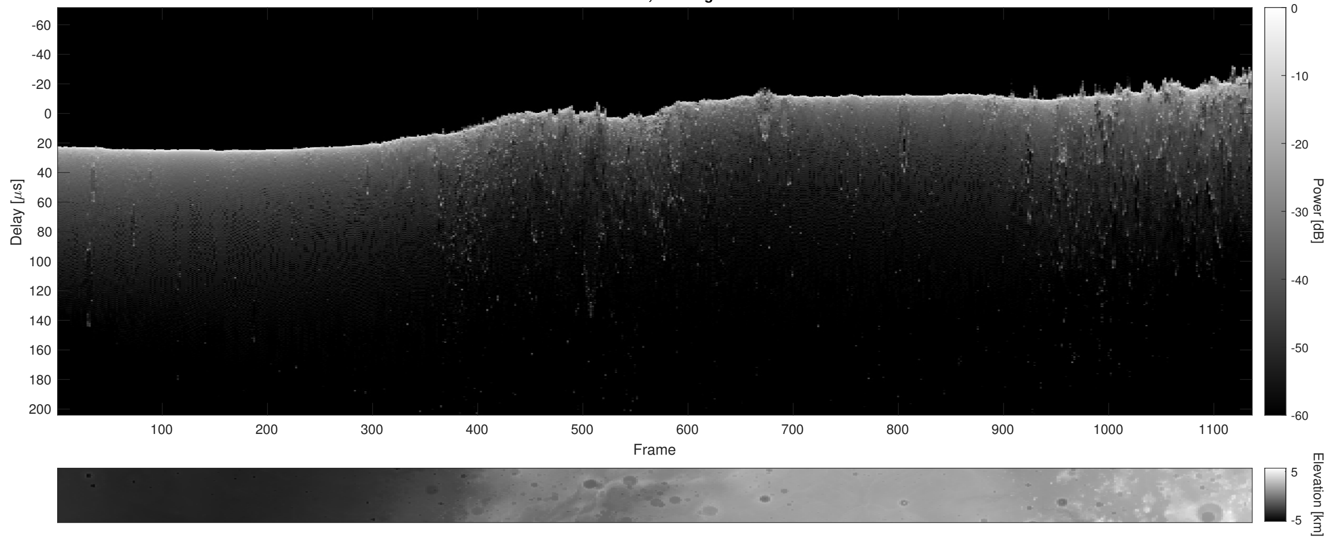
Orbit 13424, Cluttergram
