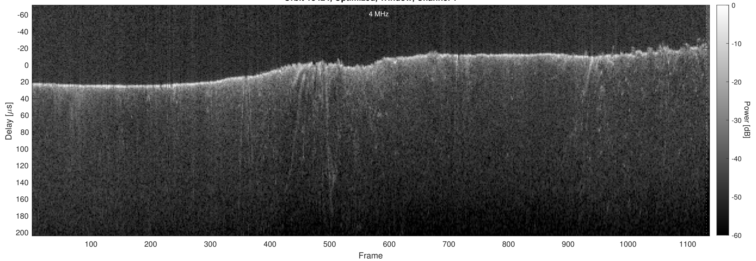
Orbit 13424, Optimized, Window, Channel 2
