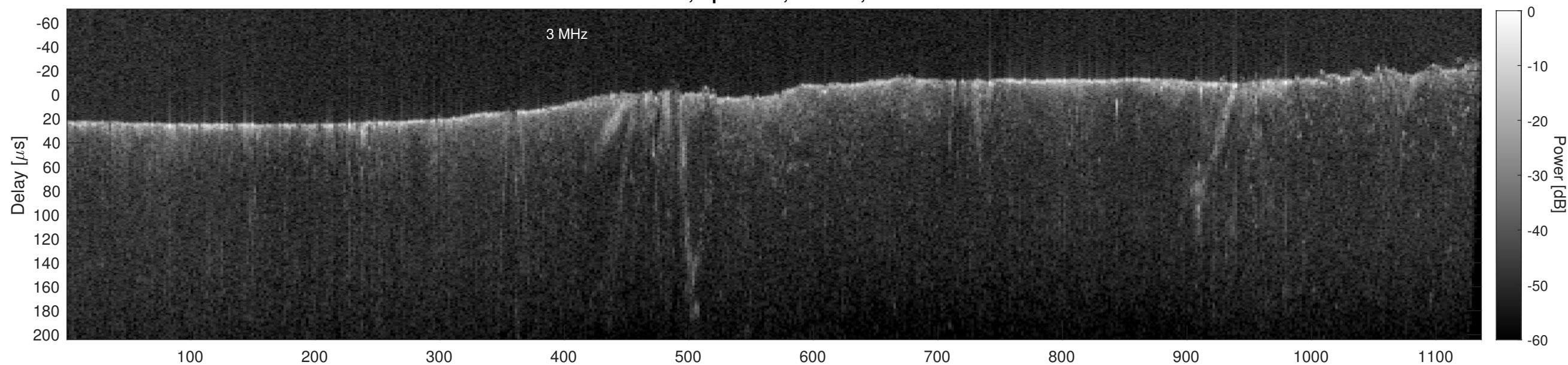
Orbit 13424, Cluttergram
