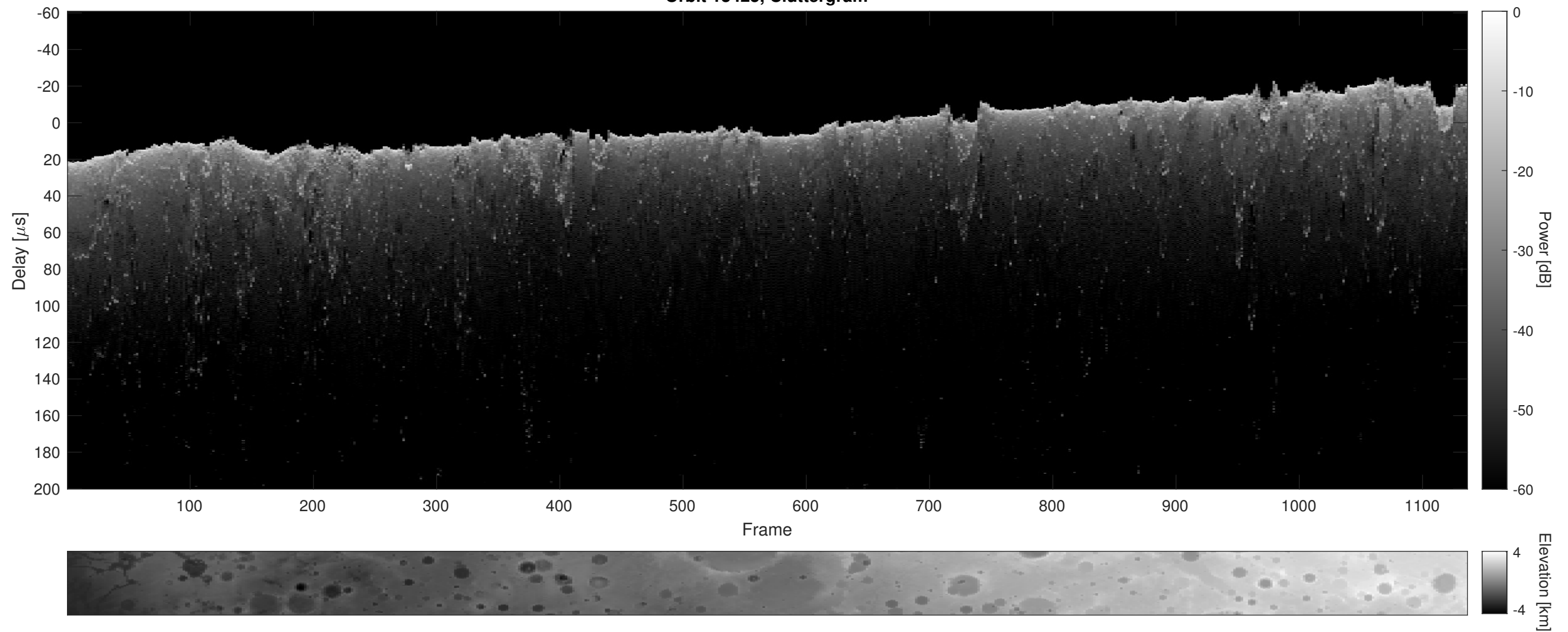
Orbit 13425, Cluttergram
