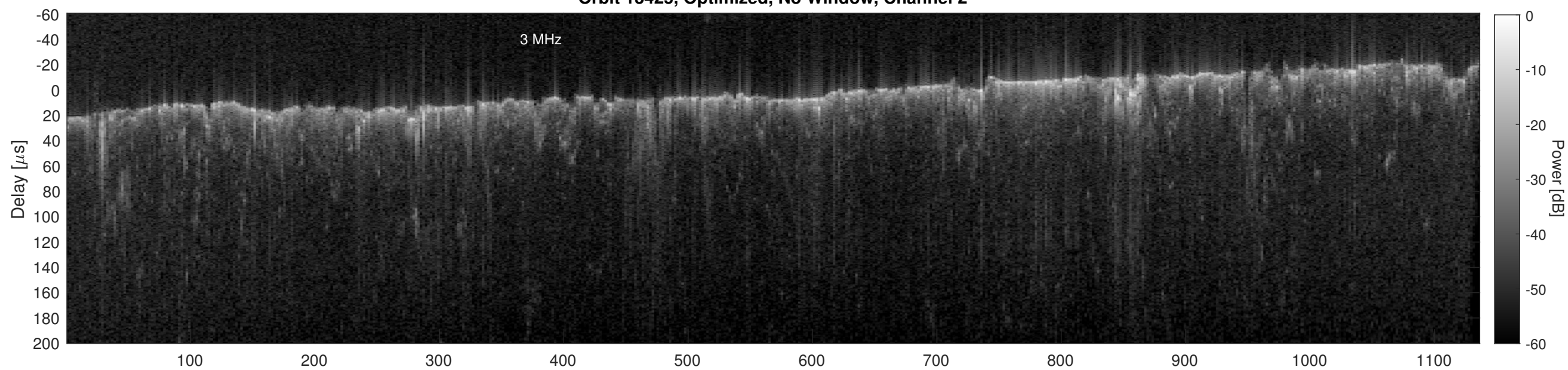
Orbit 13425, Cluttergram
