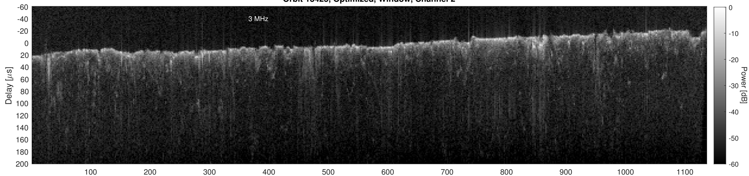
Orbit 13425, Cluttergram
