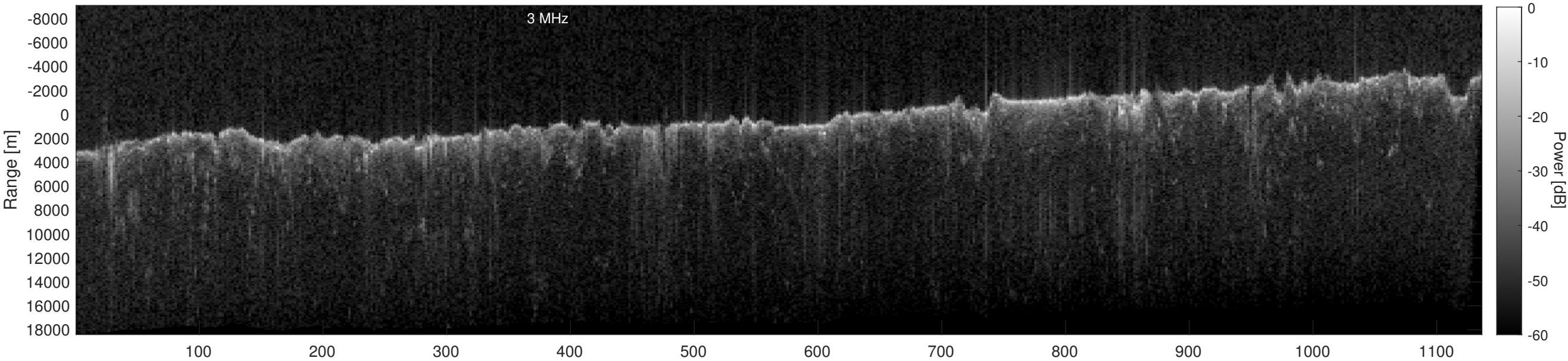
Orbit 13425, Depth-Corrected Cluttergram
