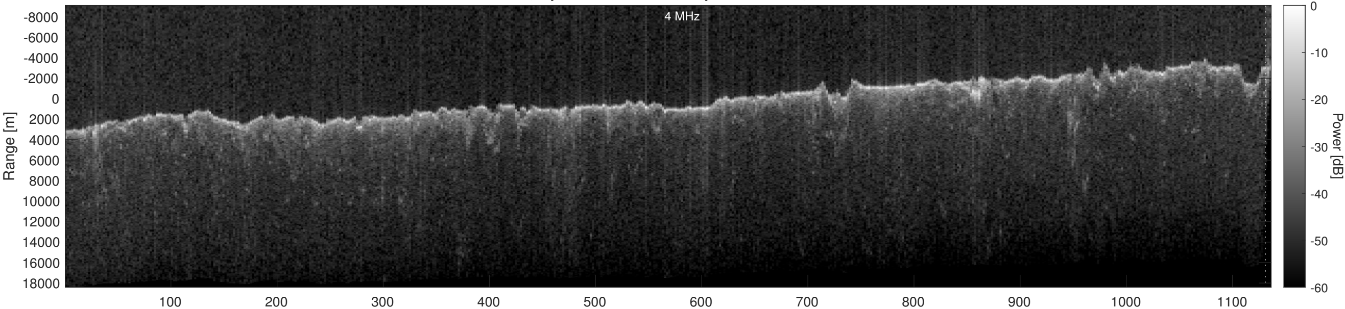
Orbit 13425, Optimized, Window, Depth-Corrected, Channel 2
