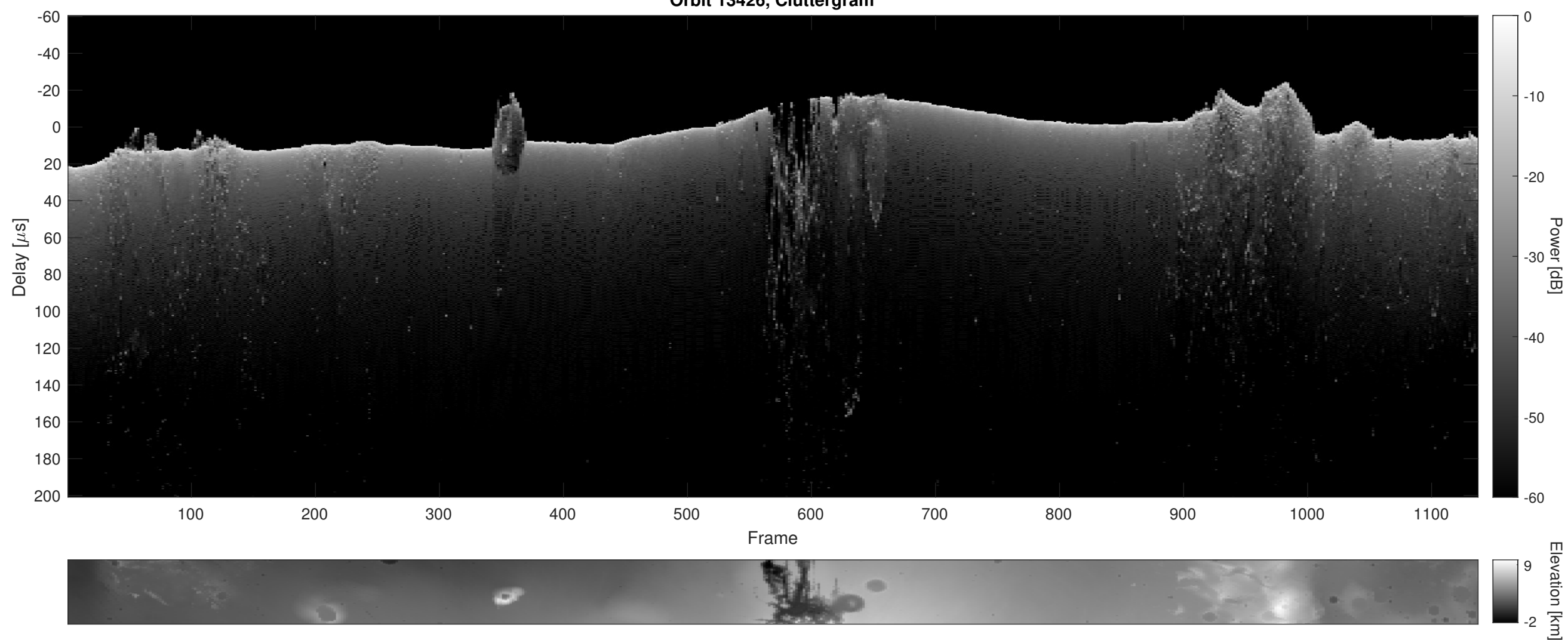
Orbit 13426, Cluttergram
