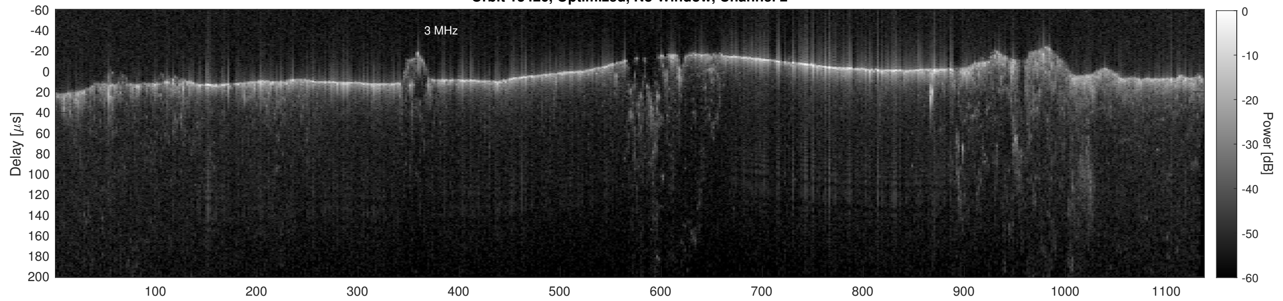
Orbit 13426, Cluttergram
